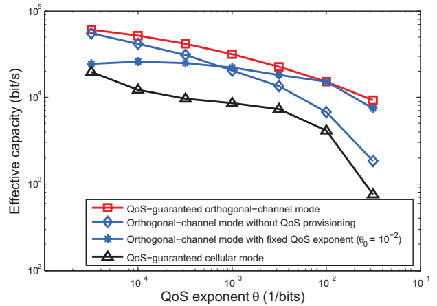
Fig. 5. Comparison of the effective capacity (corresponding to Instance 1) using our proposed QoS-driven power allocation scheme for the orthogonal-channel mode, the power allocation scheme for the orthogonal-channel mode without QoS provisioning, the power allocation scheme for the orthogonal-channel mode with fixed QoS exponent ( \theta_0 = 10^{-2} ), and the QoS-driven power allocation scheme for the cellular mode.
