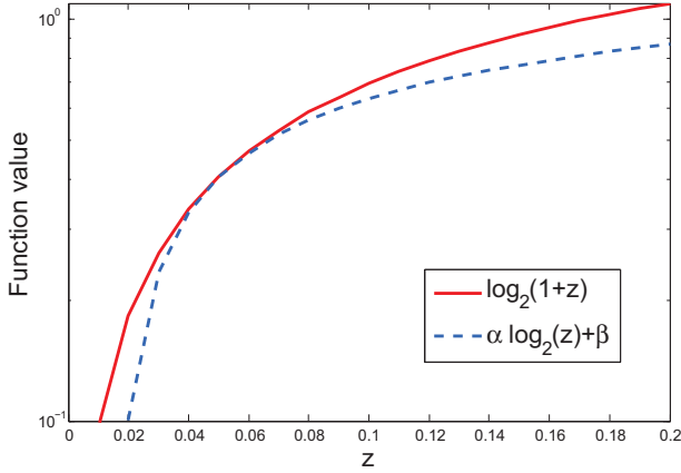
Fig. 2. The function \log_2(1+z) and its tightest lower-bound \alpha \log_2(z) + \beta with z_0 = 0.05 .
