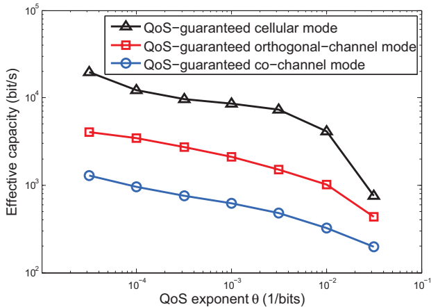
Fig. 8. Comparison of the effective capacity (corresponding to Instance 2) using the QoS-driven power allocation scheme for the cellular mode, our proposed QoS-driven power allocation scheme for the orthogonal-channel mode, and our proposed QoS-driven power allocation scheme for the co-channel mode.
