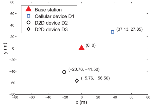
Fig. 3. Instance 1: An instance of positions of the BS, the cellular device, and the D2D pair. The coordinates of the BS, the cellular device D1, the D2D device D2, and the D2D device D3 are (0, 0), (37.13, 27.85), (-20.76, -41.50), and (-5.76, -56.50), respectively.
