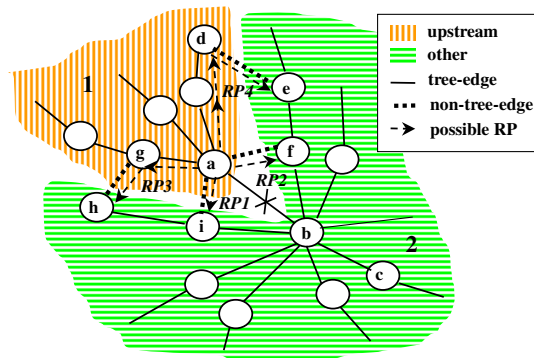
Fig. 1. The sink tree of b
