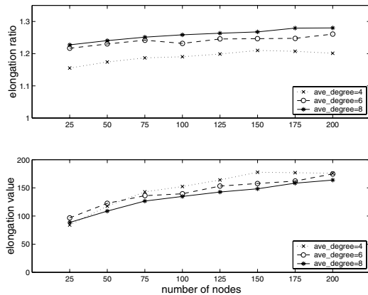
Fig. 4. Elongation ratio and value compared to optimal paths
