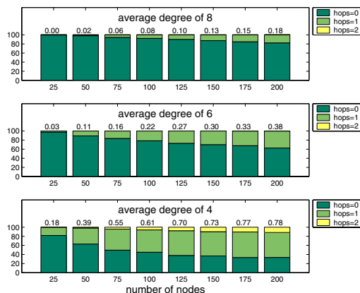
Fig. 3. Percentage of RPs with different number of signaling hops and average number of signaling hops (the number above each vertical bar)
