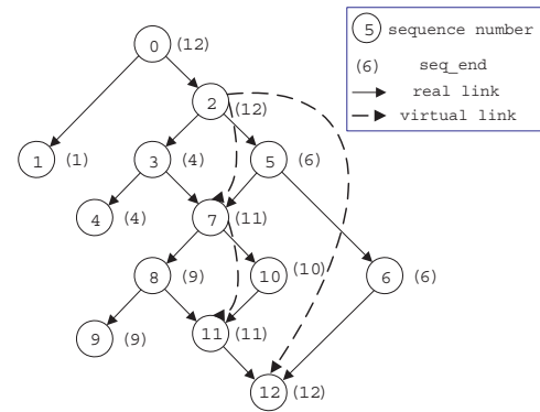
Fig. 2. Sequence numbers of nodes in a subtree tree
