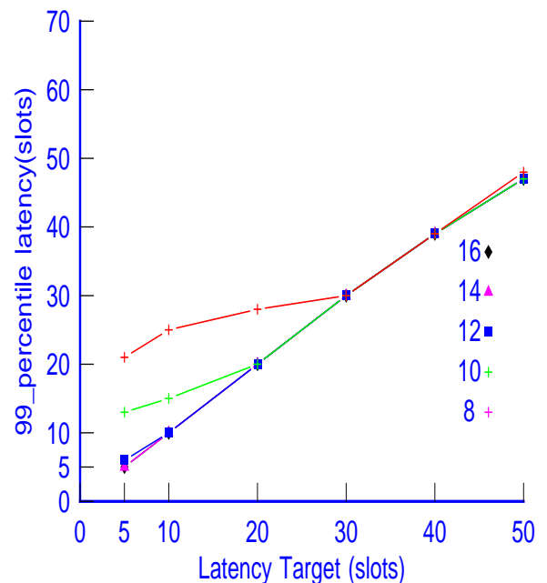
Fig. 11. Effect of the slack period.
