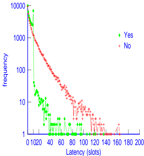
Fig. 10. Distribution of latencies with and without latency reduction.
