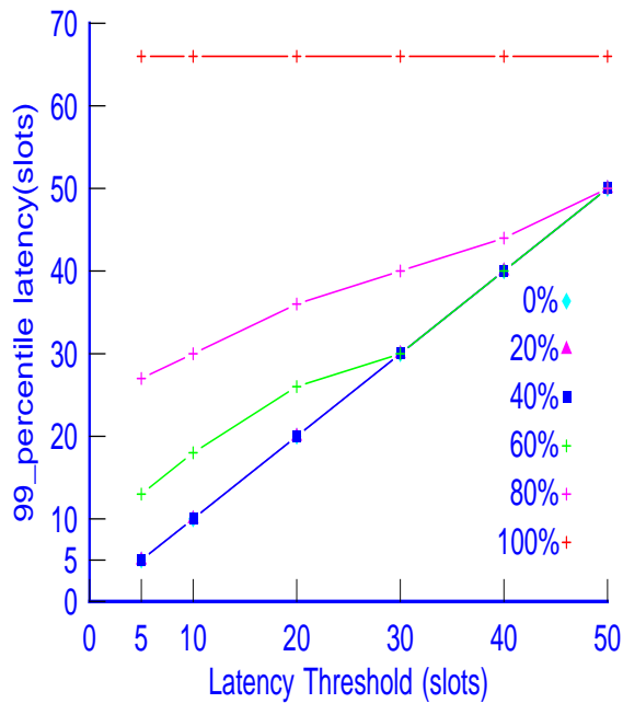
Fig. 8. Observed 99-percentile latency with backward move technique.
