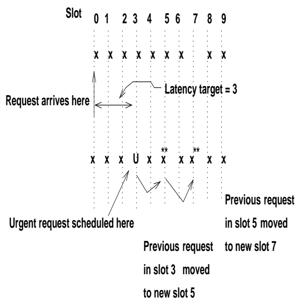
Fig. 5. Sequence of backward moves to achieve latency target.
