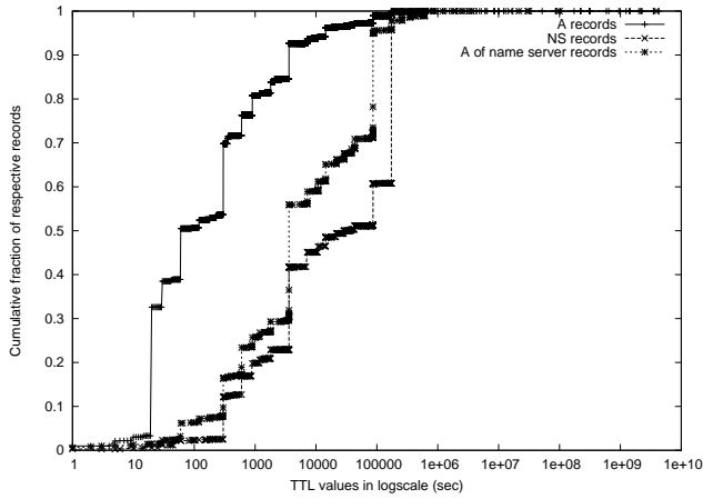
Figure 2. Cumulative Distribution Function (CDF) of TTL values for A, NS, and A of name server records.
