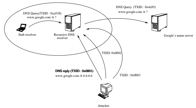
Figure 1. DNS cache poisoning scenario.
