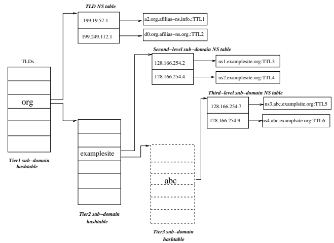
Figure 4. MiND query verifying data structure.
