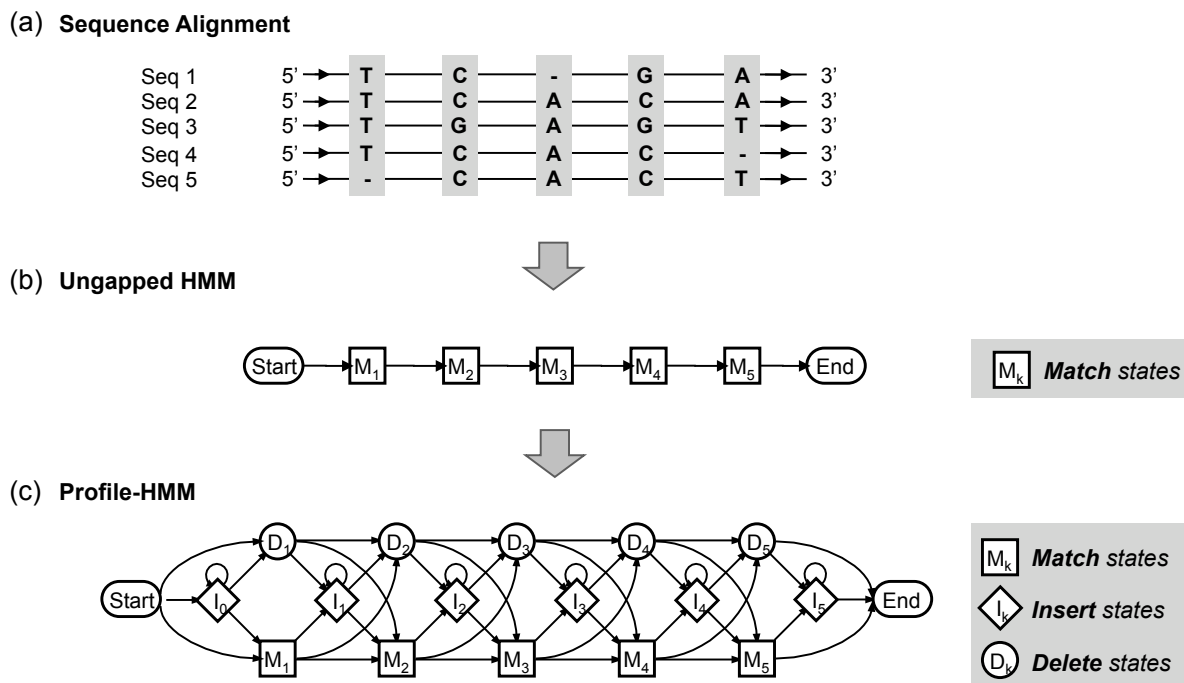
Fig. 2. Profile hidden Markov model. (a) Multiple sequence alignment for constructing the profile-HMM. (b) The ungapped HMM that represents the consensus sequence of the alignment. (c) The final profile-HMM that allows insertions and deletions.
