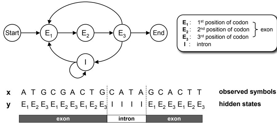
Fig. 1. A simple HMM for modeling eukaryotic genes.
