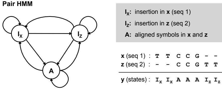
Fig. 3. Example of a pair hidden Markov model. A pair-HMM generates an aligned pair of sequences. In this example, two DNA sequences \mathbf{x} and \mathbf{z} are simultaneously generated by the pair-HMM, where the underlying state sequence is \mathbf{y} . Note that the state sequence \mathbf{y} uniquely determines the pairwise alignment between \mathbf{x} and \mathbf{z} .
