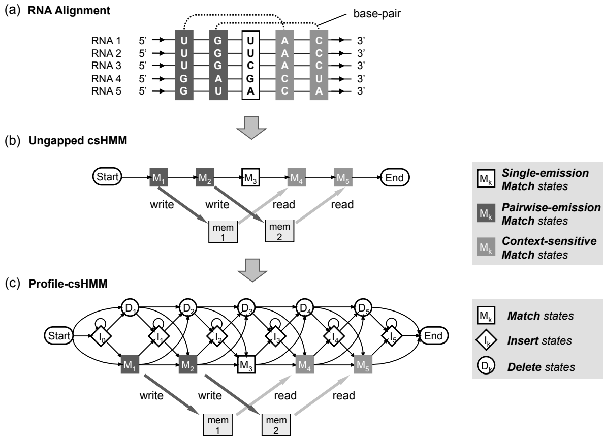
Fig. 5. Constructing a profile-csHMM from a multiple RNA sequence alignment. (a) Example of an RNA sequence alignment. The consensus RNA structure has two base-pairs. (b) An ungapped csHMM constructed from the given alignment. (c) The final profile-csHMM that can handle symbol matches, insertions, and deletions.
